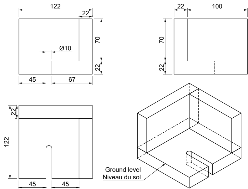
Figure 6: Right fixed beacon support (Modèle A)
